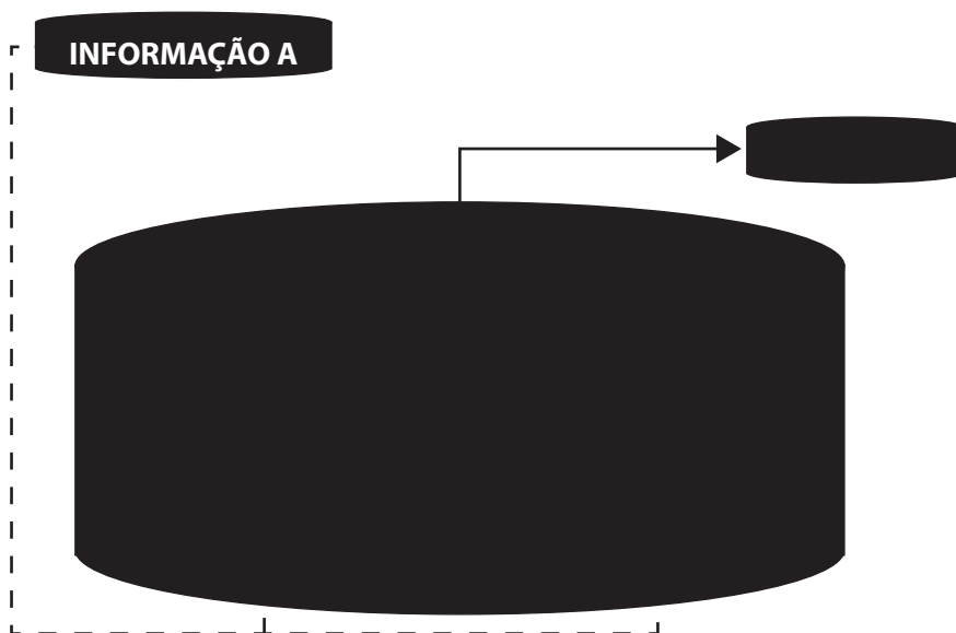
Fig. 38 - RAID 0.
